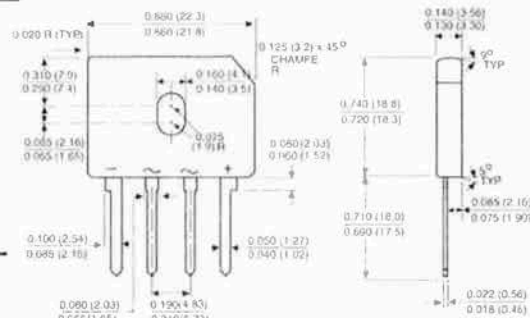
Polarity shown in front side of case, positive lead by beveled corner
