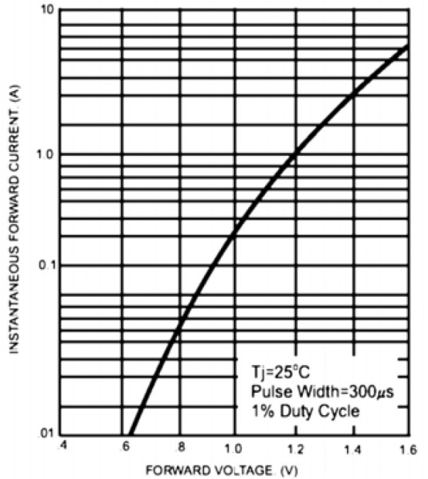
FIG.5- TYPICAL FORWARD CHARACTERISTICS
