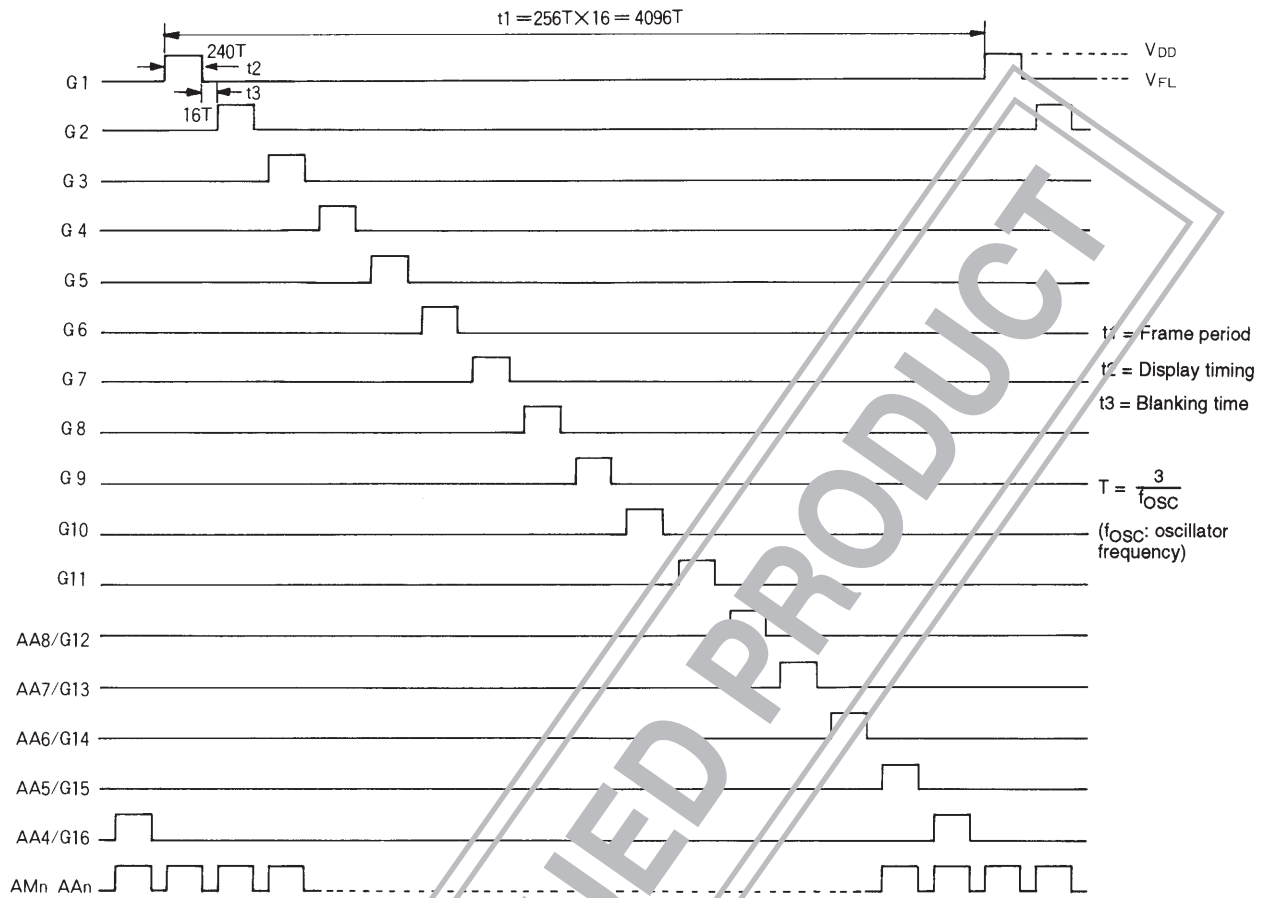
Fig. 3 Gate Timing Chart (16 display digits)
