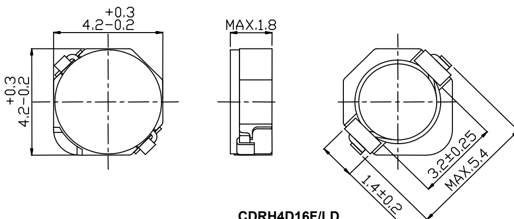
CDRH4D16F/LD
