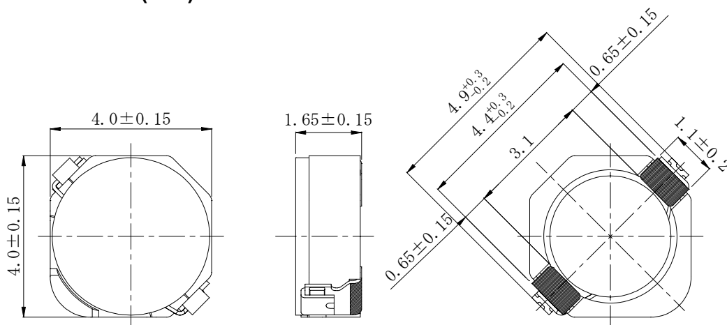
CDRH4D16FB ELECTRODE
