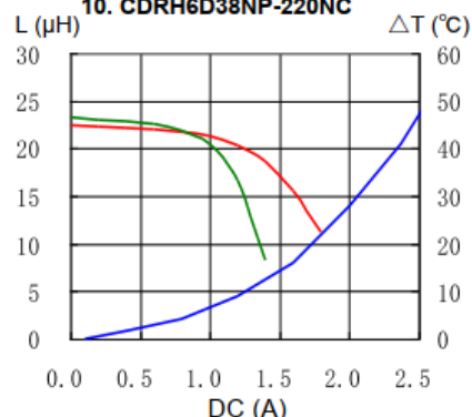
10. CDRH6D38NP-220NC
