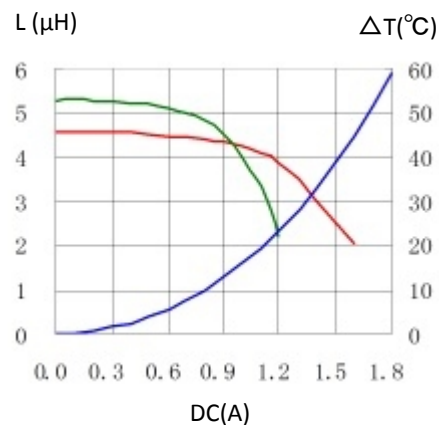
3. CDRH40D18ANP-4R7NC
