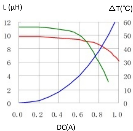
5. CDRH40D18ANP-100NC
