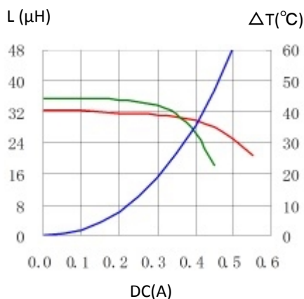
8. CDRH40D18ANP-330NC
