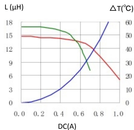
6. CDRH40D18ANP-150NC
