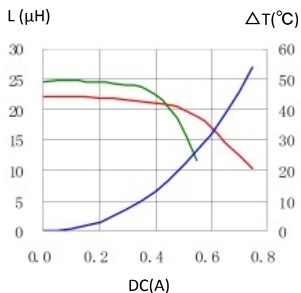
7. CDRH40D18ANP-220NC
