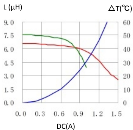
4. CDRH40D18ANP-6R8NC
