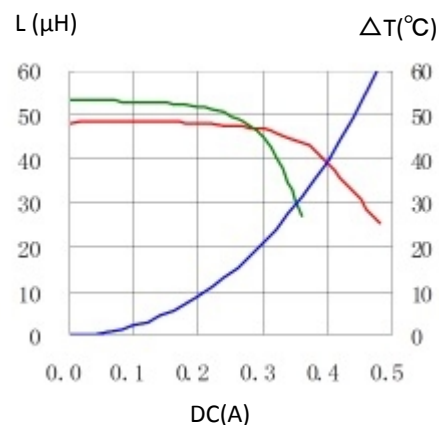
9. CDRH40D18ANP-470NC
