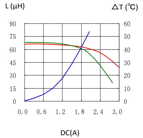
CDRH124NP-680MC
