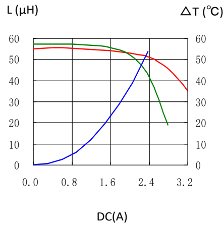
CDRH124NP-560MC
