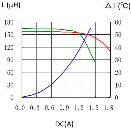
CDRH124NP-151MC
