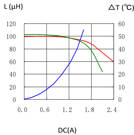
CDRH124NP-101MC
