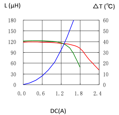
CDRH124NP-121MC
