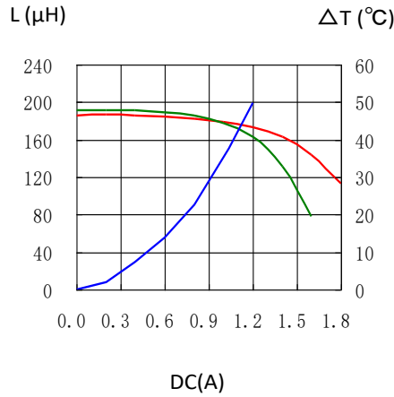
CDRH124NP-181MC
