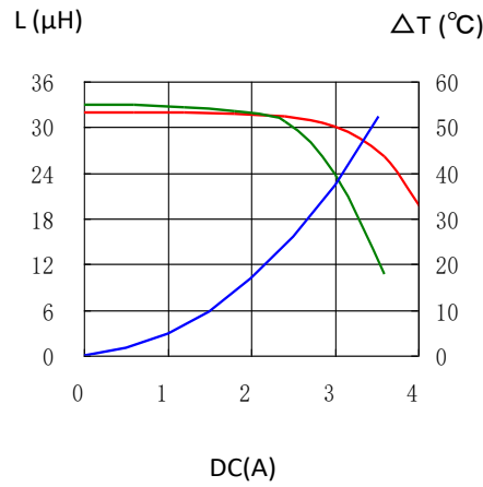
CDRH124NP-330MC
