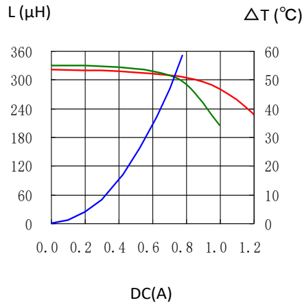
CDRH124NP-331MC
