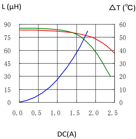
CDRH124NP-820MC
