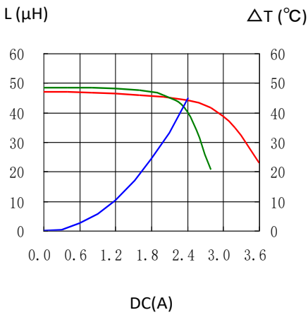
CDRH124NP-470MC
