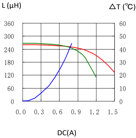
CDRH124NP-271MC
