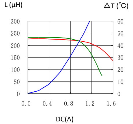
CDRH124NP-221MC
