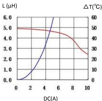
5. CDMPIH10D38NP-4R7PC
