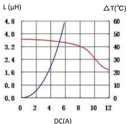
4. CDMPIH10D38NP-3R6PC
