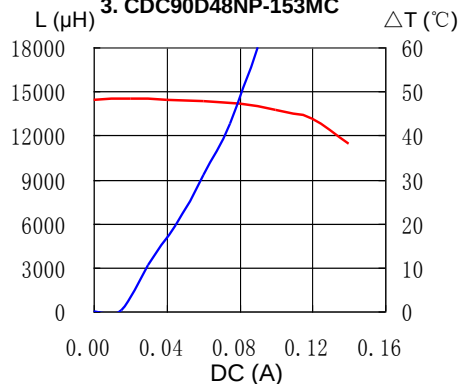
3. CDC90D48NP-153MC
