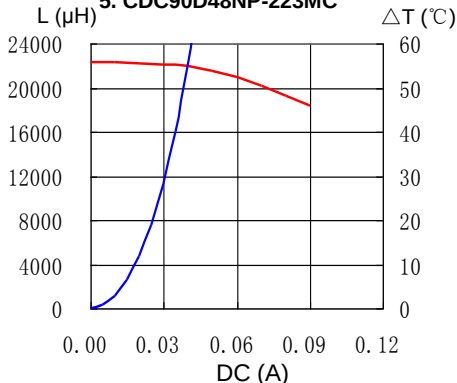
5. CDC90D48NP-223MC
