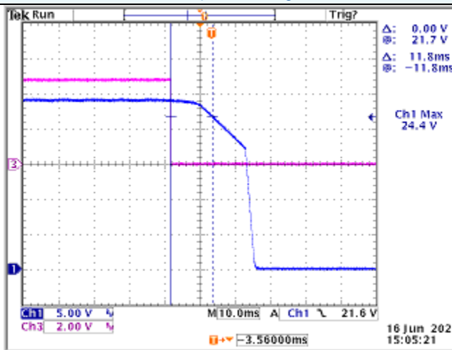
Hold-up Time Test @100Vac/60Hz
