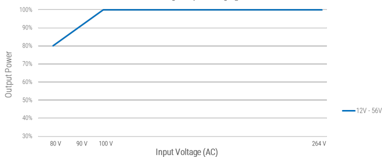
Power Derating vs Input Voltage @40°C
