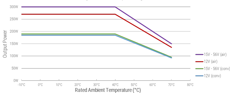
Power Derating vs Ambient Temperature @Vin>100 Vac
