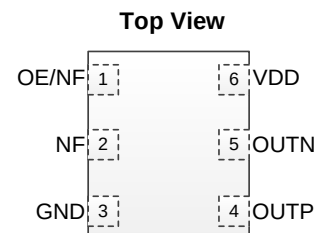
Figure 3. Pin Assignments
