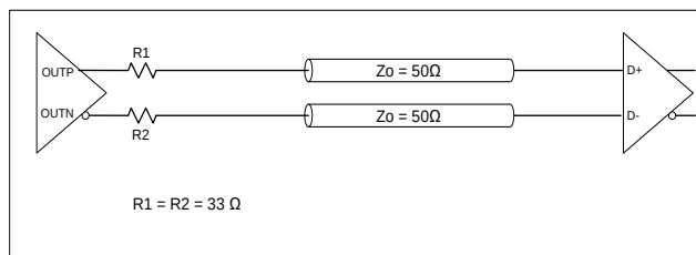
Figure 32. Low-power HCSL Termination
