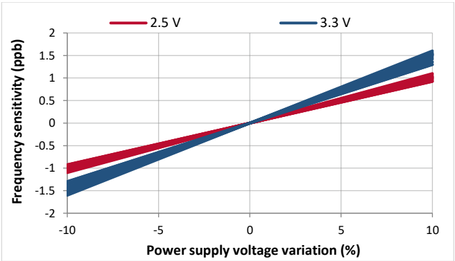
Figure 23. VDD sensitivity
