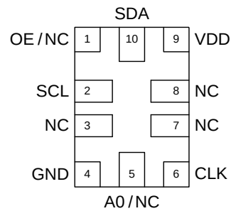
Figure 5. DCTCXO
