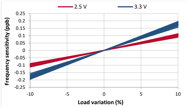
Figure 22. Load sensitivity
