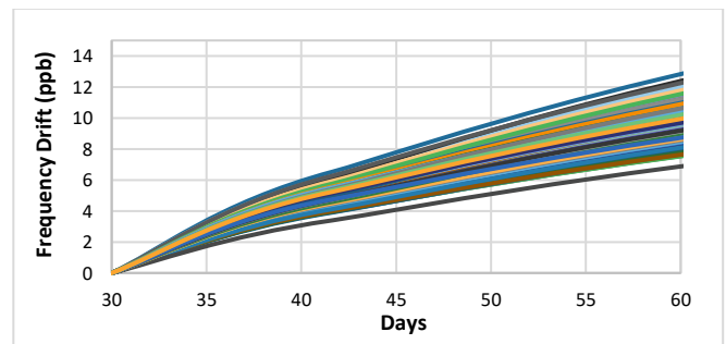
Figure 21. Frequency drift after 30 days [16]
