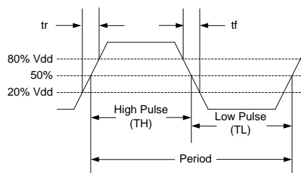
Figure 3. Waveform
