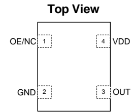
Figure 1. Pin Assignments
