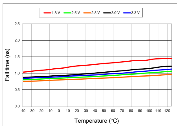
Figure 12. 20%-80% Fall Time vs Temperature
