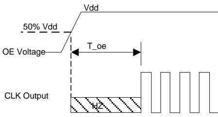
Figure 17. OE Enable Timing (OE Mode Only)
