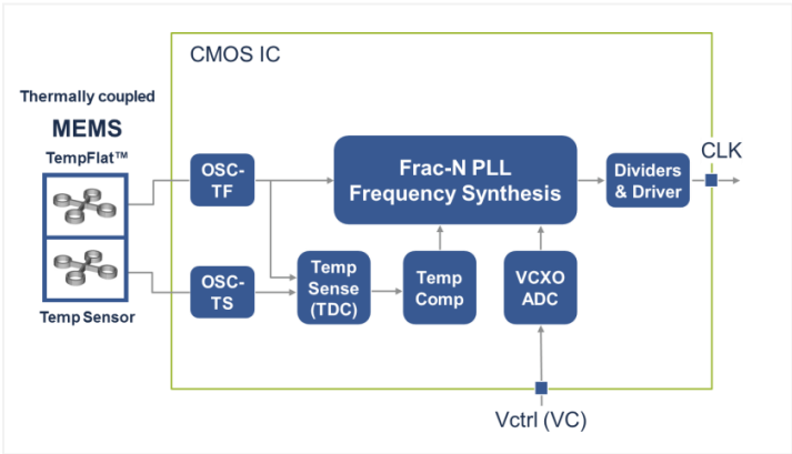
Figure 22. Block Diagram - VCTCXO
