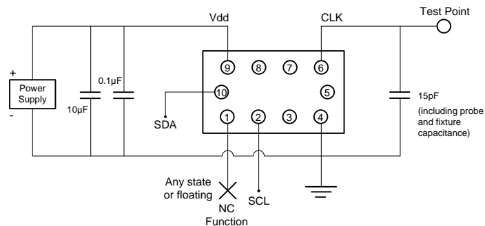
Figure 12. LVCMOS Test Circuit (I²C Control)
