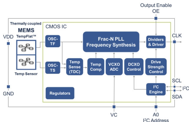
Figure 19. Elite Architecture
