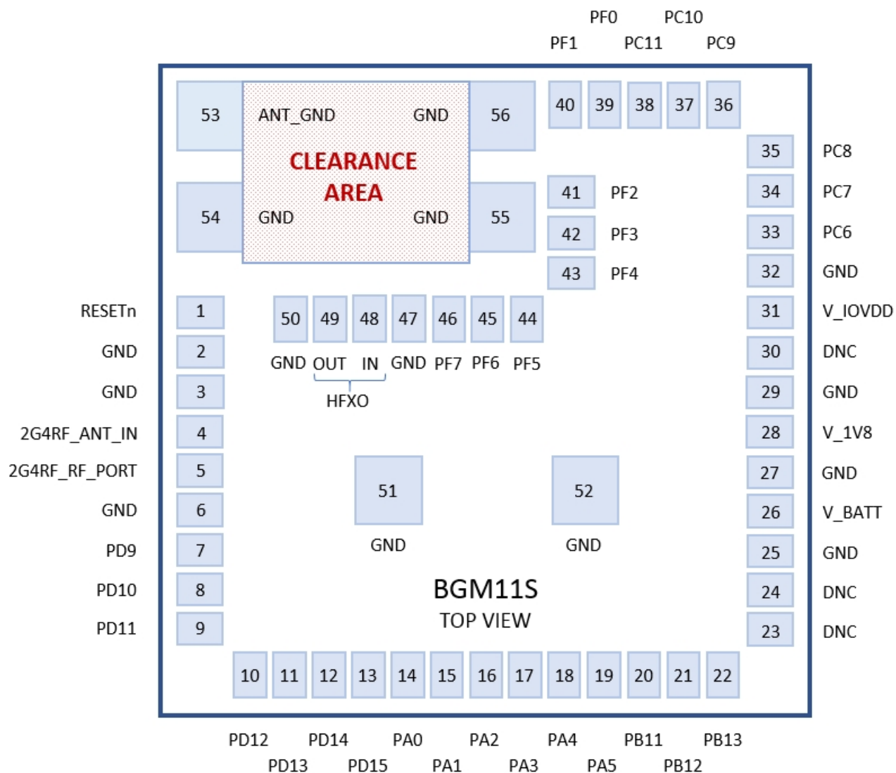
Figure 7.1. BGM11S Pinout
