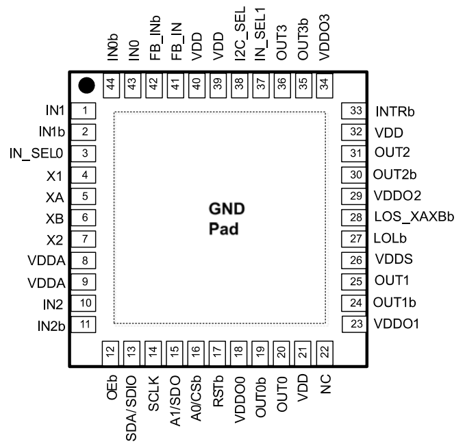
Si 5340 44QFN Top View
