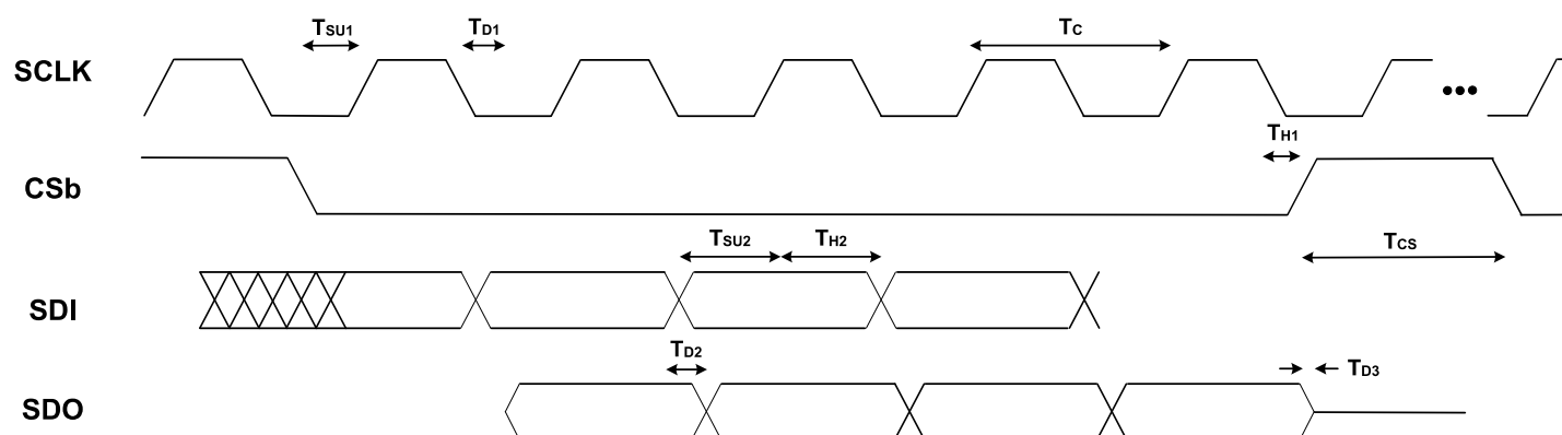
Figure 5.2. 4-Wire SPI Serial Interface Timing
