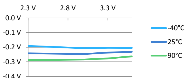
Figure 8: Output Voltage – V_{DD} versus supply voltage when sourcing 8mA
