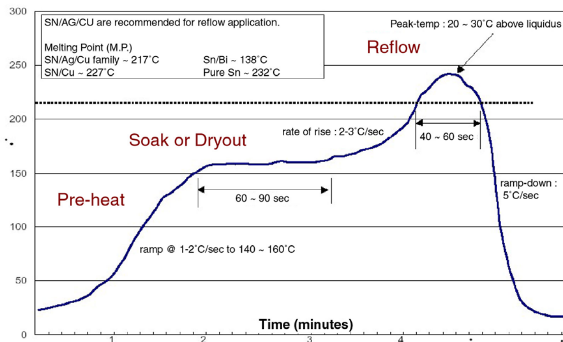
Figure 18 Recommended Reflow Temperature Profile
