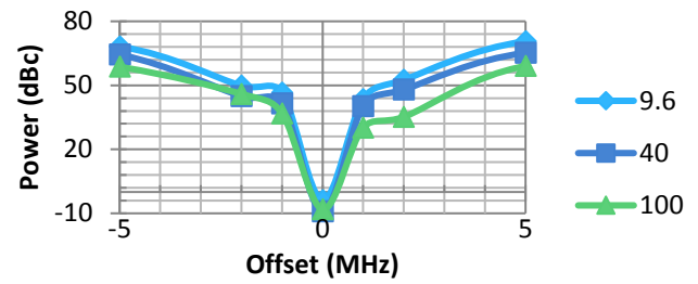
Figure 6: Typical Blocking performance
