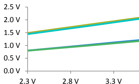
Figure 9: Input threshold voltages incl. hysteresis, versus supply voltage
