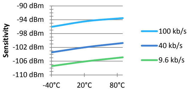
Figure 5: Typical Sensitivity (average over process corners)
