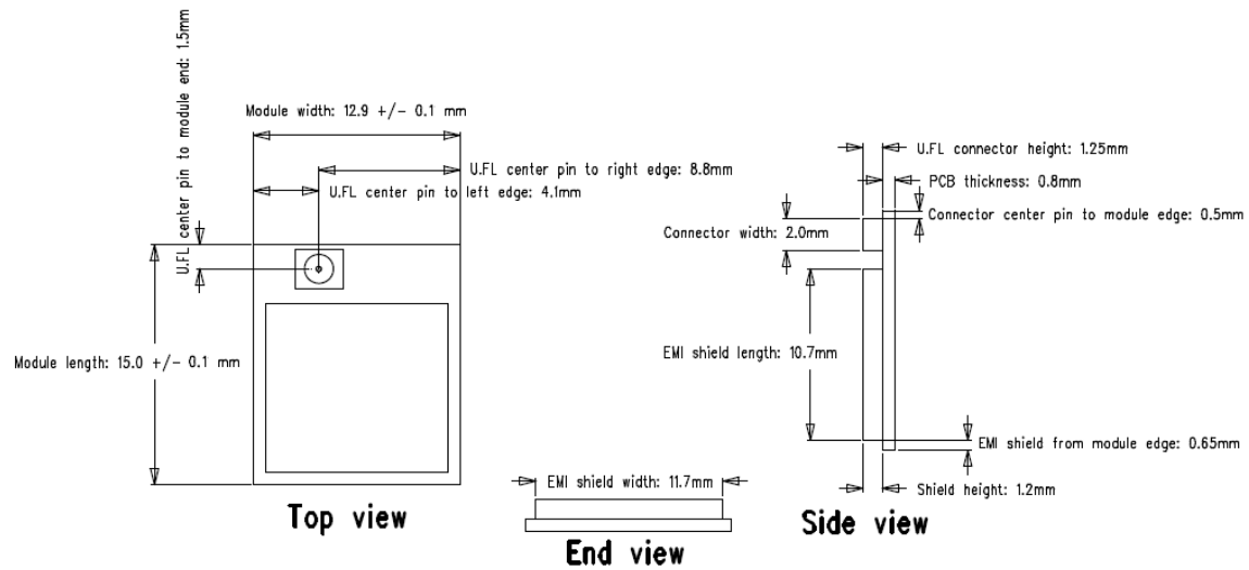
Figure 8.1. BGM111E Package Dimensions
