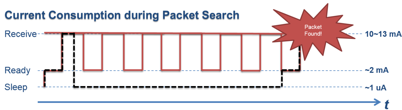
Figure 12. Preamble Sense Mode
