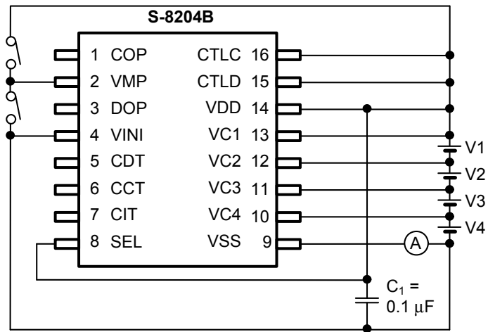
Figure 4 Test Circuit 1
