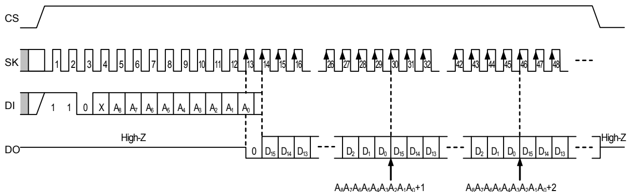
Figure 6 Read Timing
