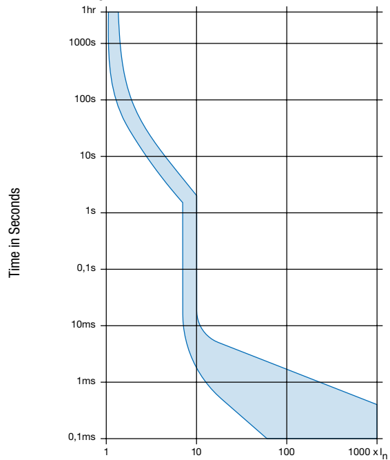
Version G / Magnetic 6-10 xIn
