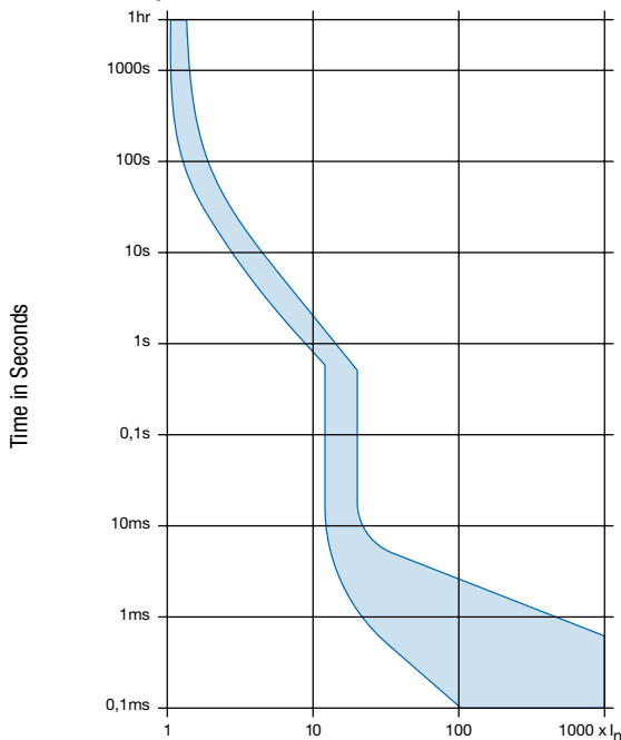
Version H / Magnetic 12-20 xIn
