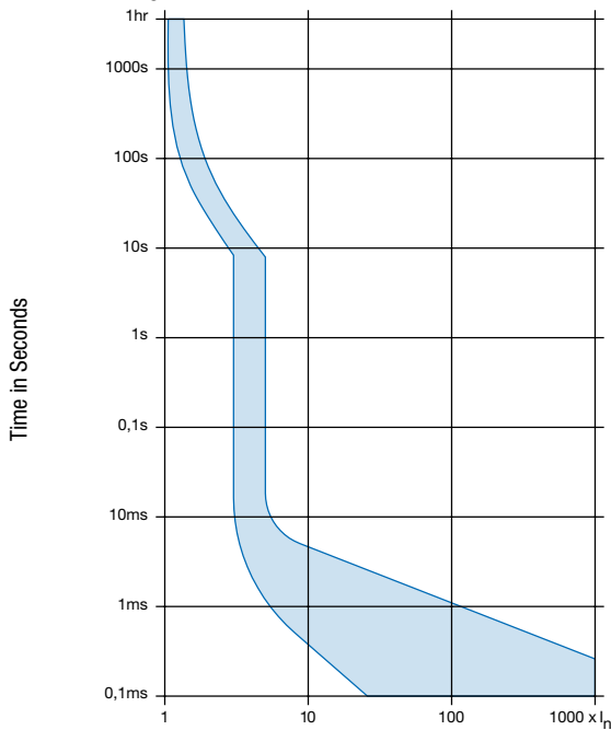
Version F / Magnetic 3-5 xIn
