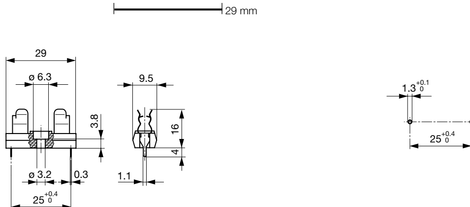
Drilling diagram
