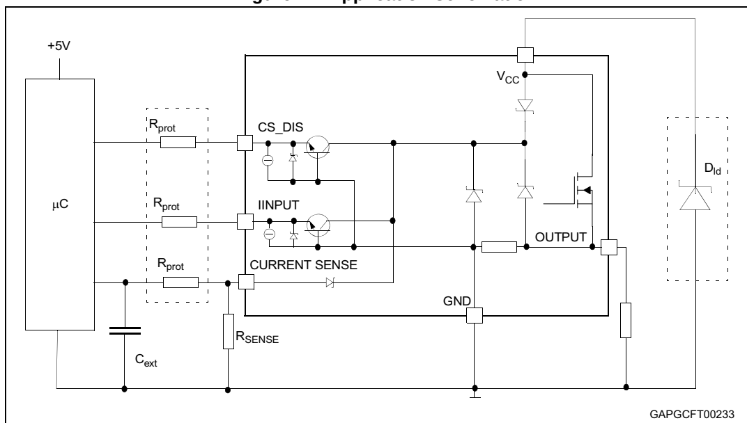
Figure 22. Application schematic
