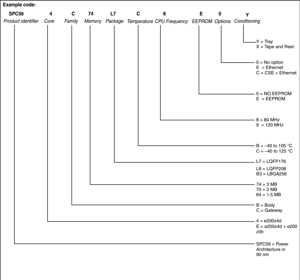
Figure 39. Ordering information scheme
