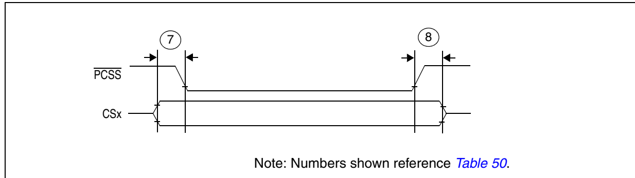
Figure 32. DSPI PCS strobe ( \overline{\text{PCSS}} ) timing
