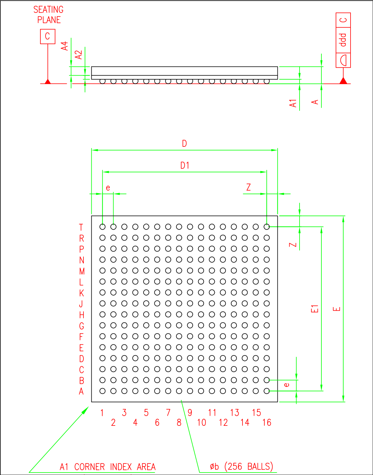
Figure 38. LBGA256 mechanical drawing
