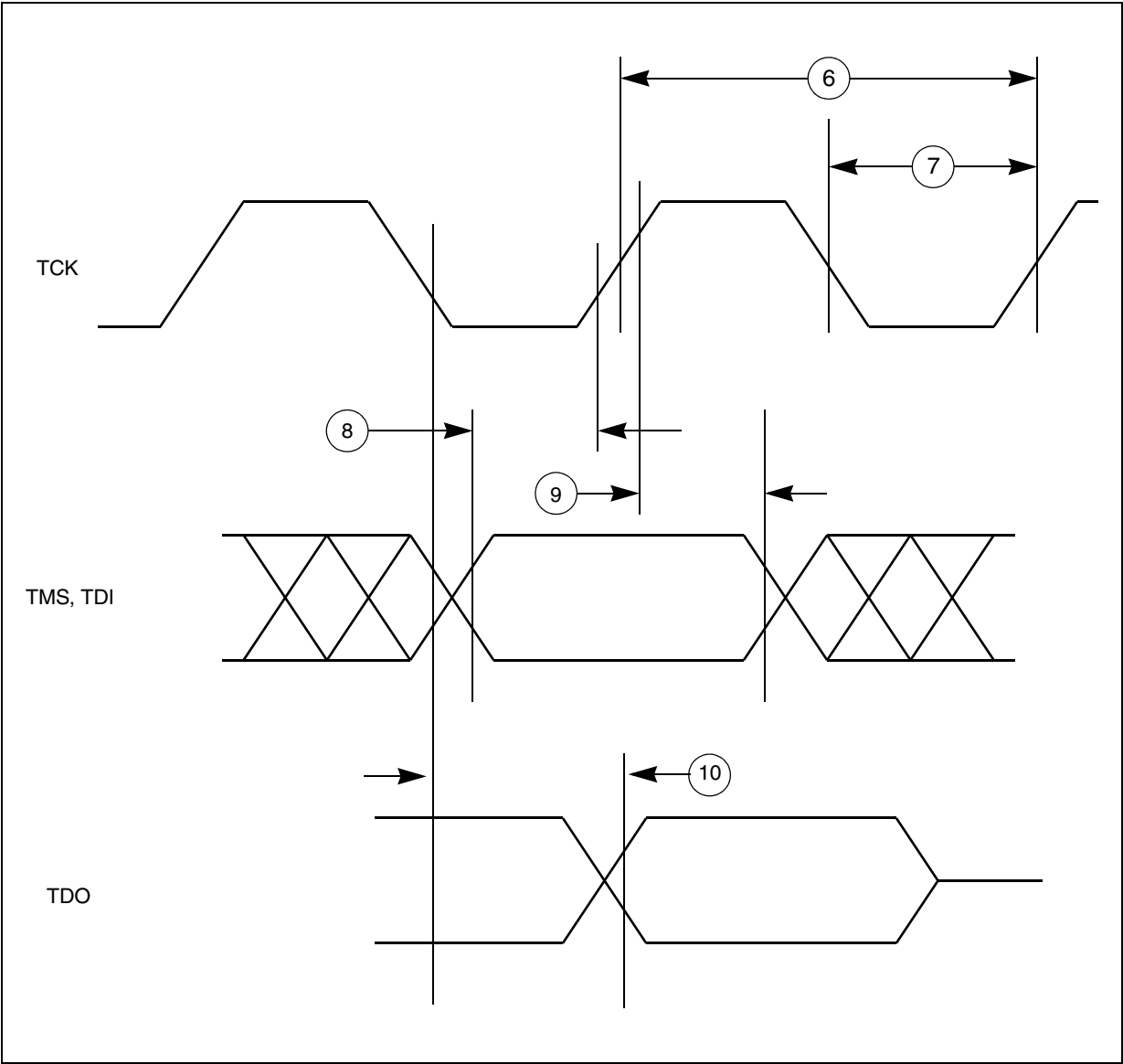
Figure 34. Nexus TDI, TMS, TDO timing
