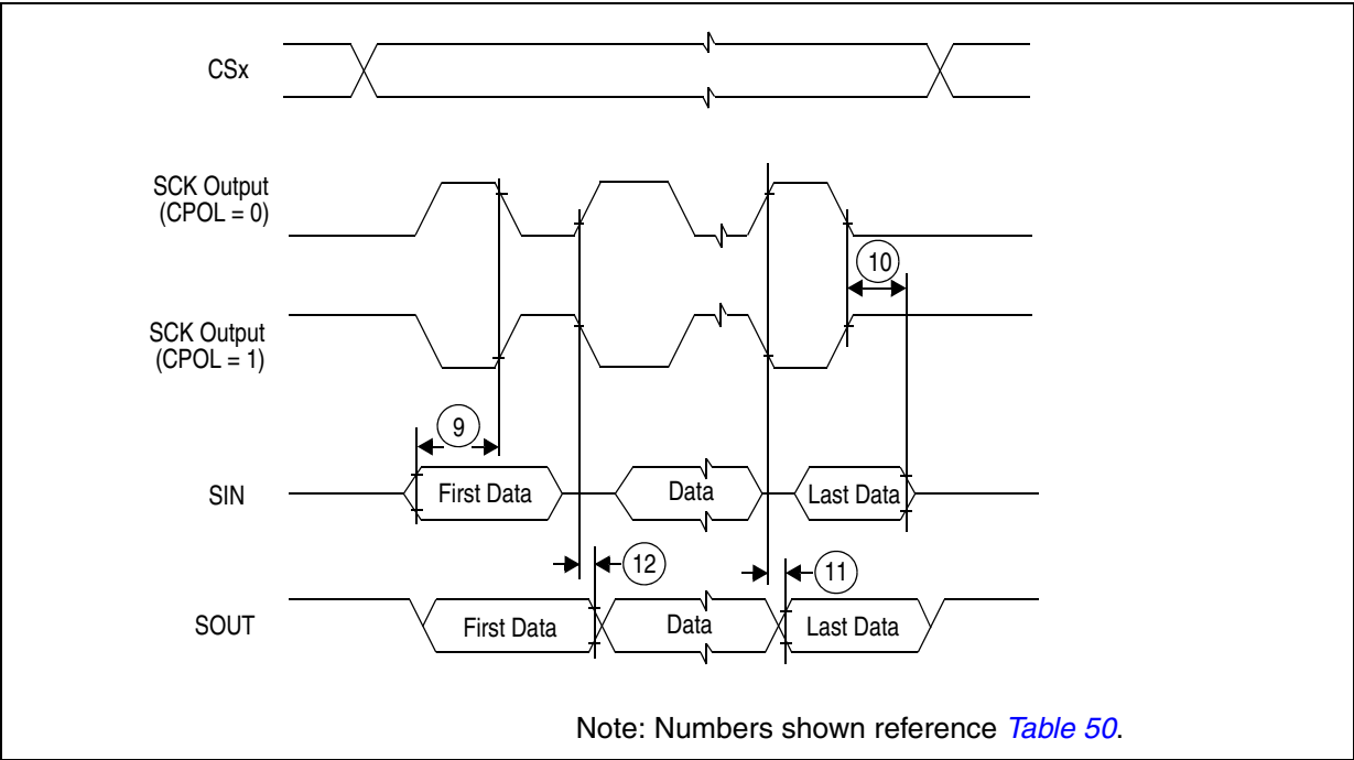
Figure 25. DSPI classic SPI timing–master, CPHA = 1
