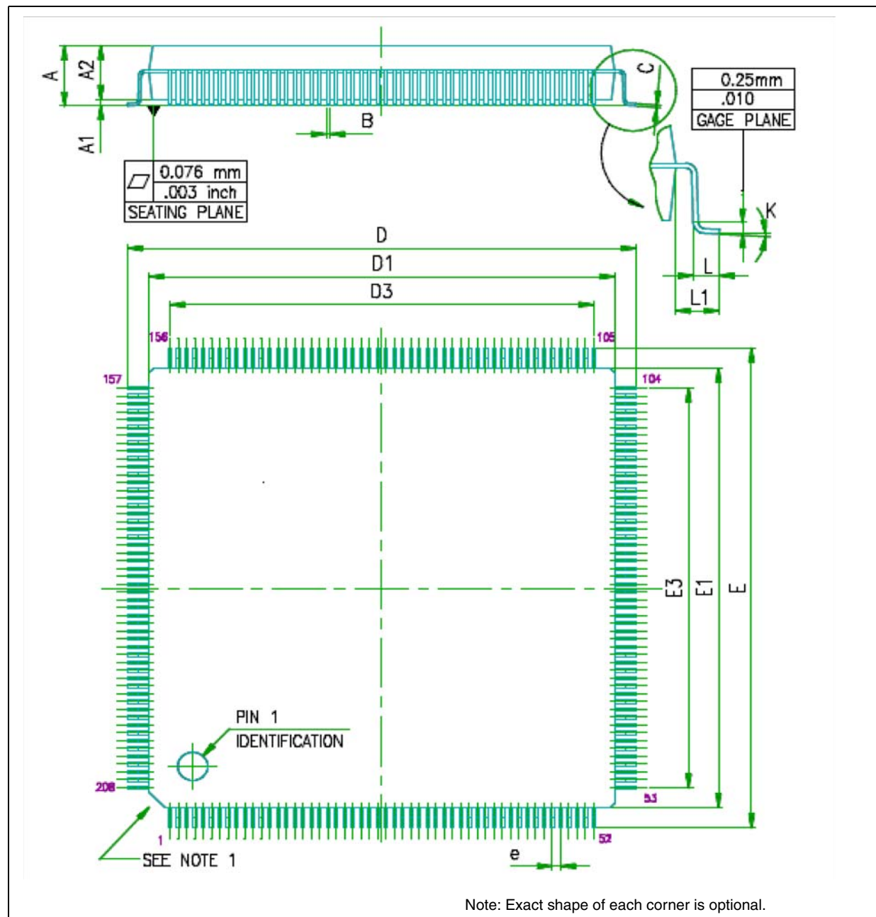
Figure 37. LQFP208 mechanical drawing
