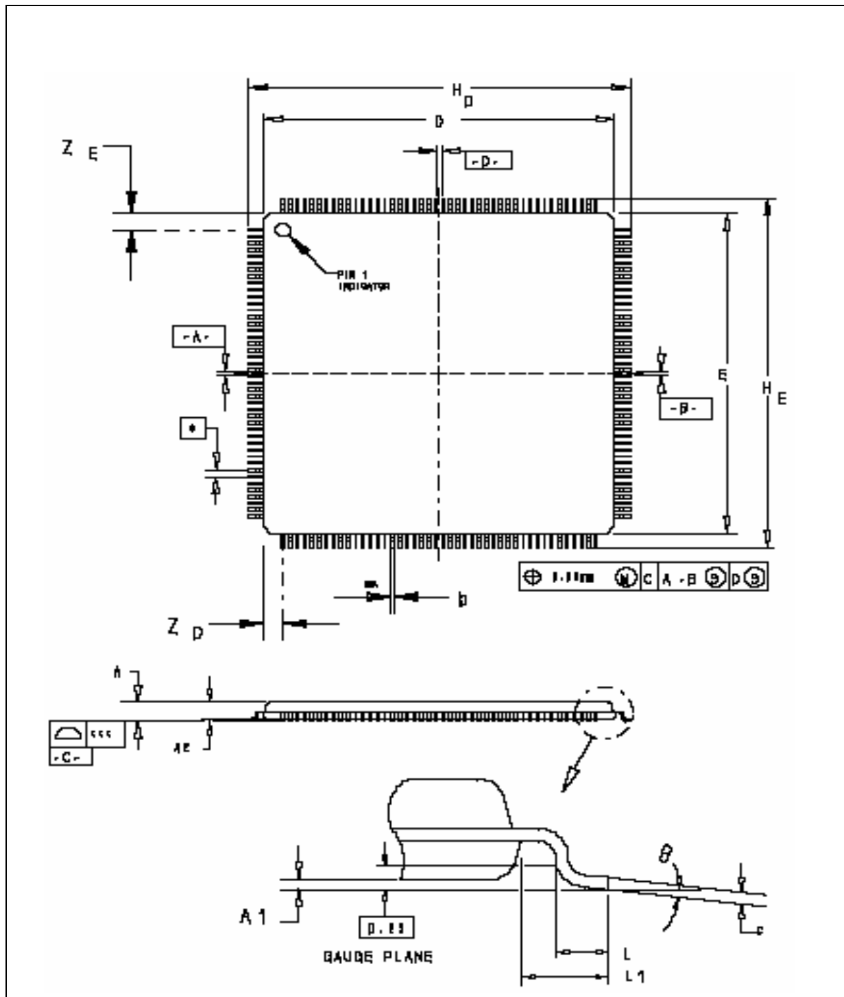
Figure 36. LQFP176 package mechanical drawing
