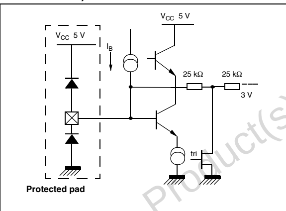
Figure 8. Average clamped video inputs (pin 8)
