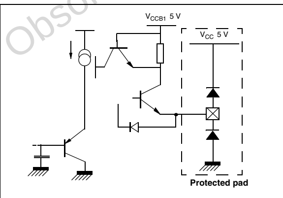
Figure 12. Video outputs (pins 36, 38, 40, 42, 44, 46, and 48)
