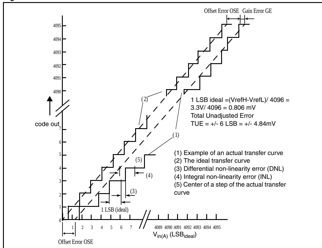
Figure 7. ADC characteristics and error definitions
