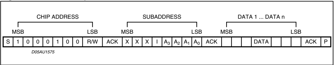
Figure 6. Interface protocol
