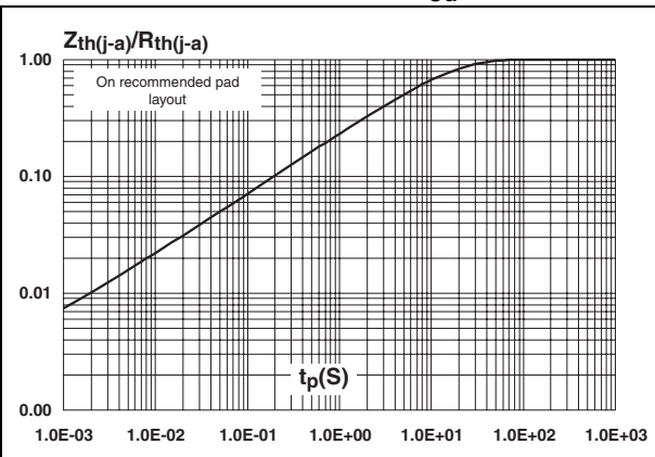
Figure 8. Relative variation of thermal impedance junction to ambient versus pulse duration (printed circuit board FR4, S_{Cu} = 1 cm 2 )
