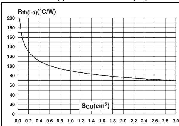
Figure 9. Thermal resistance junction to ambient versus copper surface under each lead (printed circuit board FR4, copper thickness = 35 μm)
