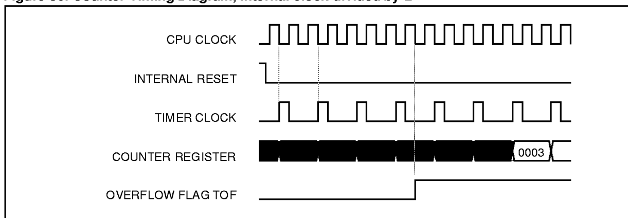
Figure 36. Counter Timing Diagram, internal clock divided by 2
