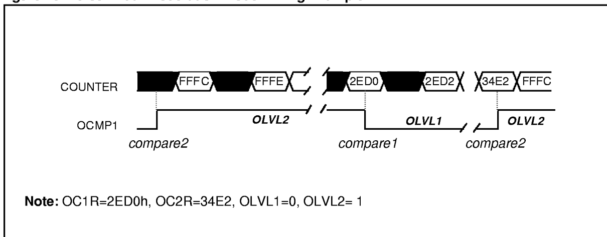
Figure 45. Pulse Width Modulation Mode Timing Example
