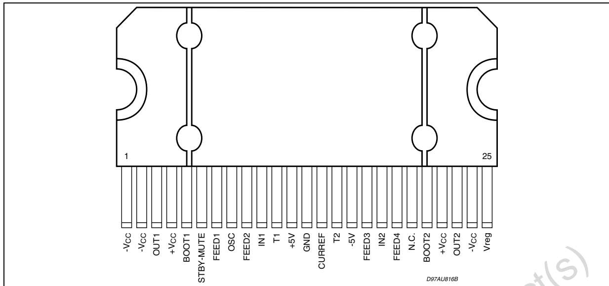
Figure 4. Pin Connection
