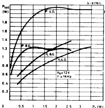
Figure 18. Total power dissipation and efficiency vs. output power
