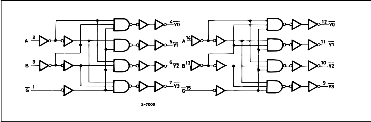
Figure 3: Logic Diagram
