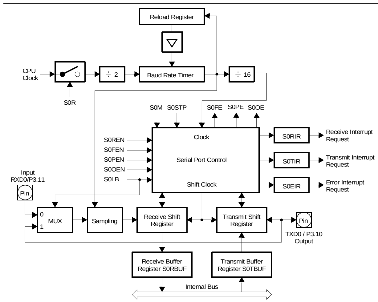
Figure 44 : Asynchronous Mode of Serial Channel ASC0
