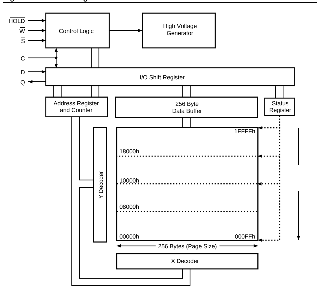
Figure 6. Block Diagram
