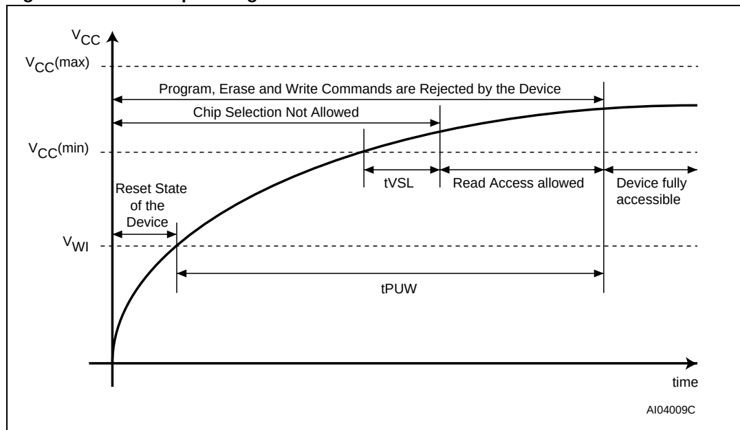
Figure 20. Power-up Timing
