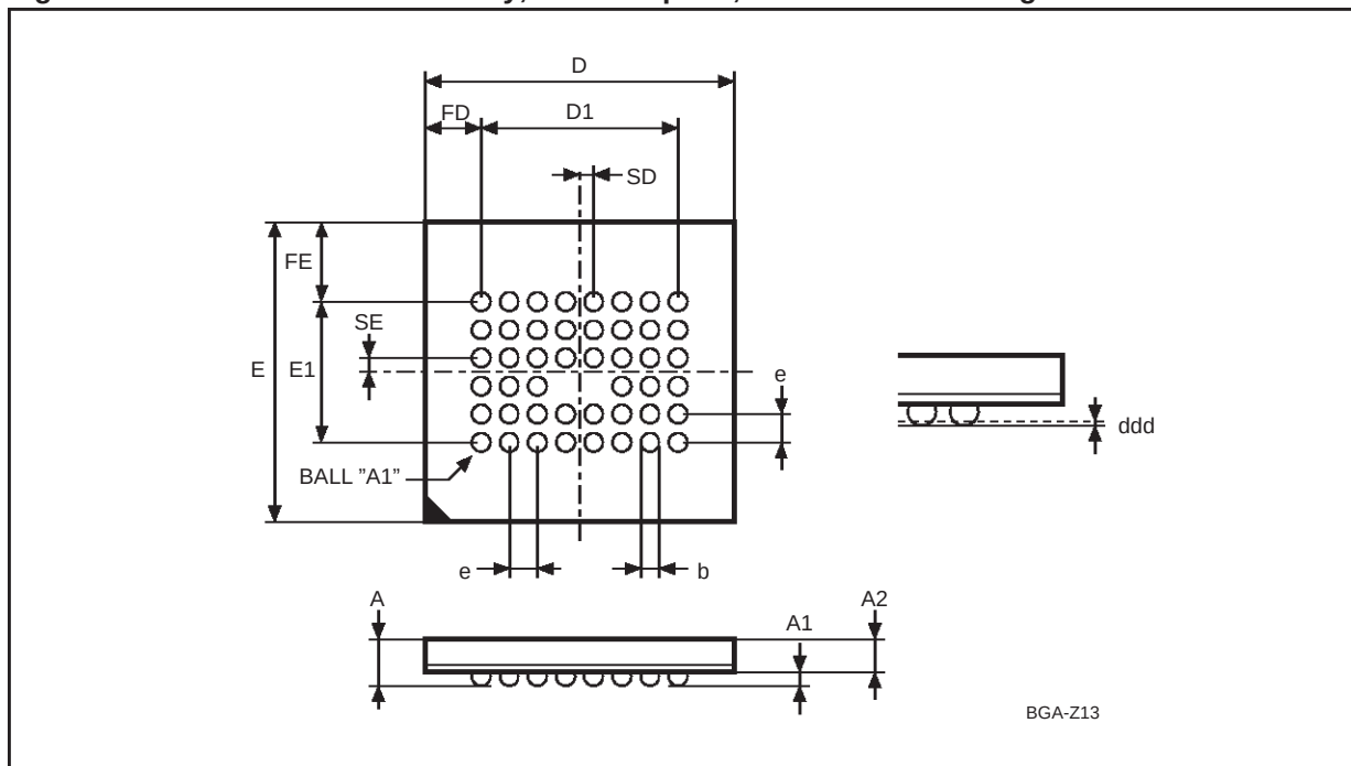
Figure 14. TFBGA46 - 8 x 6 ball array, 0.75 mm pitch, Bottom View Package Outline
