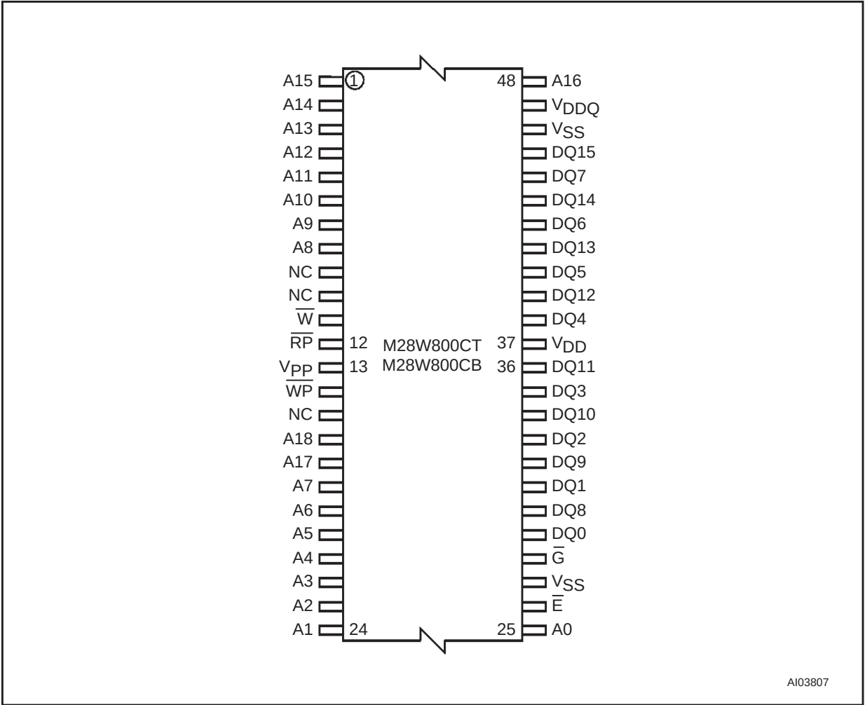
Figure 3. TSOP Connections
