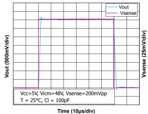
Figure 34. Large signal response with V_{CC} = 5\text{ V}
