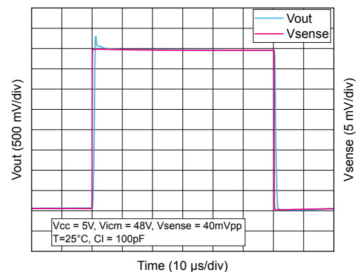
Figure 36. Large signal response with V_{CC} = 5\text{ V} (TSC2022)
