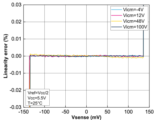
Figure 22. Linearity vs. V_{sense} with V_{CC} = 5.5 V
