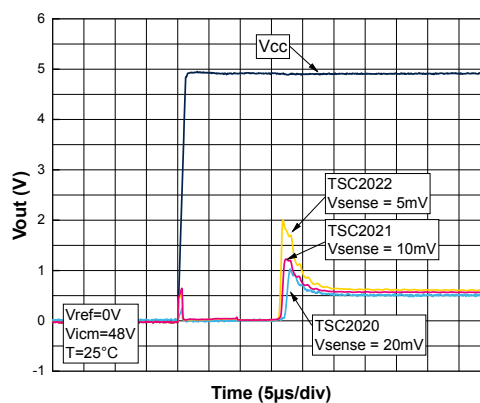
Figure 50. Power up time delay
