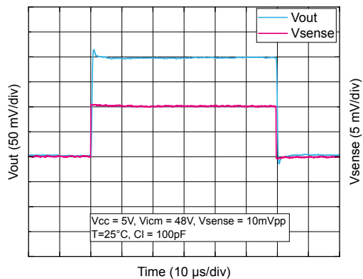
Figure 33. Small signal response with V_{CC} = 5\text{ V}
