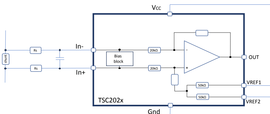
Figure 62. Input filter
