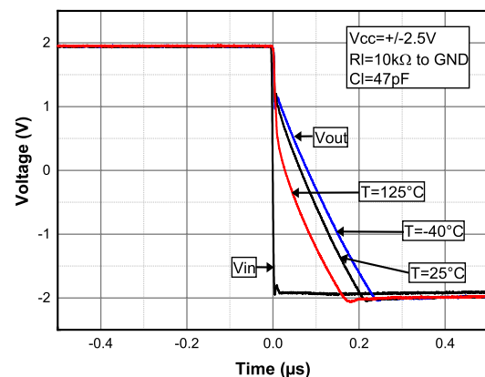
Figure 22. Negative slew rate at V_{CC} = 5\text{ V}
