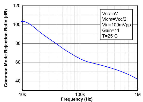
Figure 42. CMRR vs. frequency at V_{CC} = 5V
