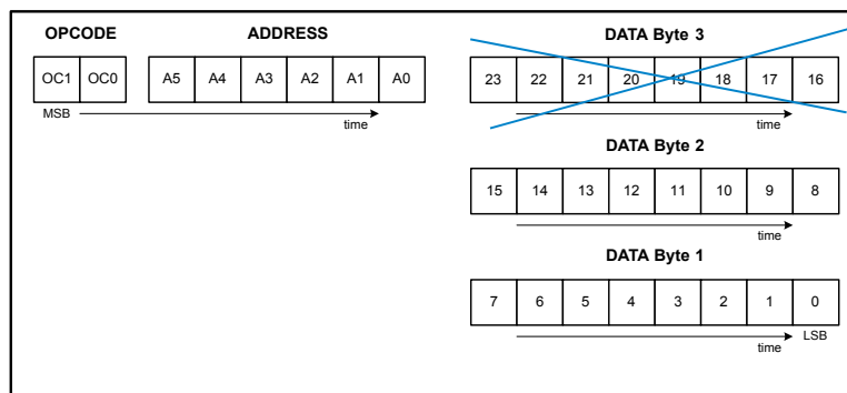
Figure 15. SDI frame
