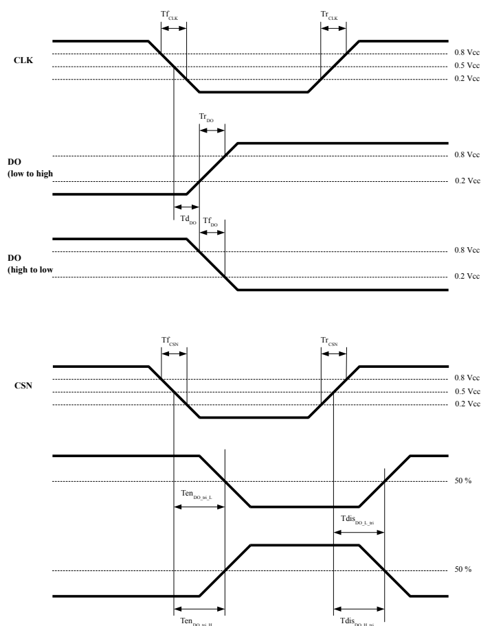
Figure 22. SPI output timing
