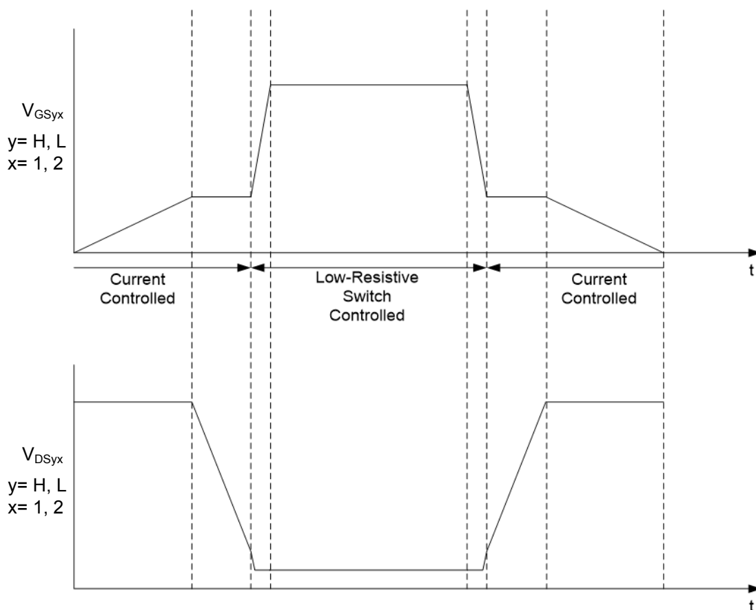
Figure 5. Full-bridge GSHx and GSLx slopes
