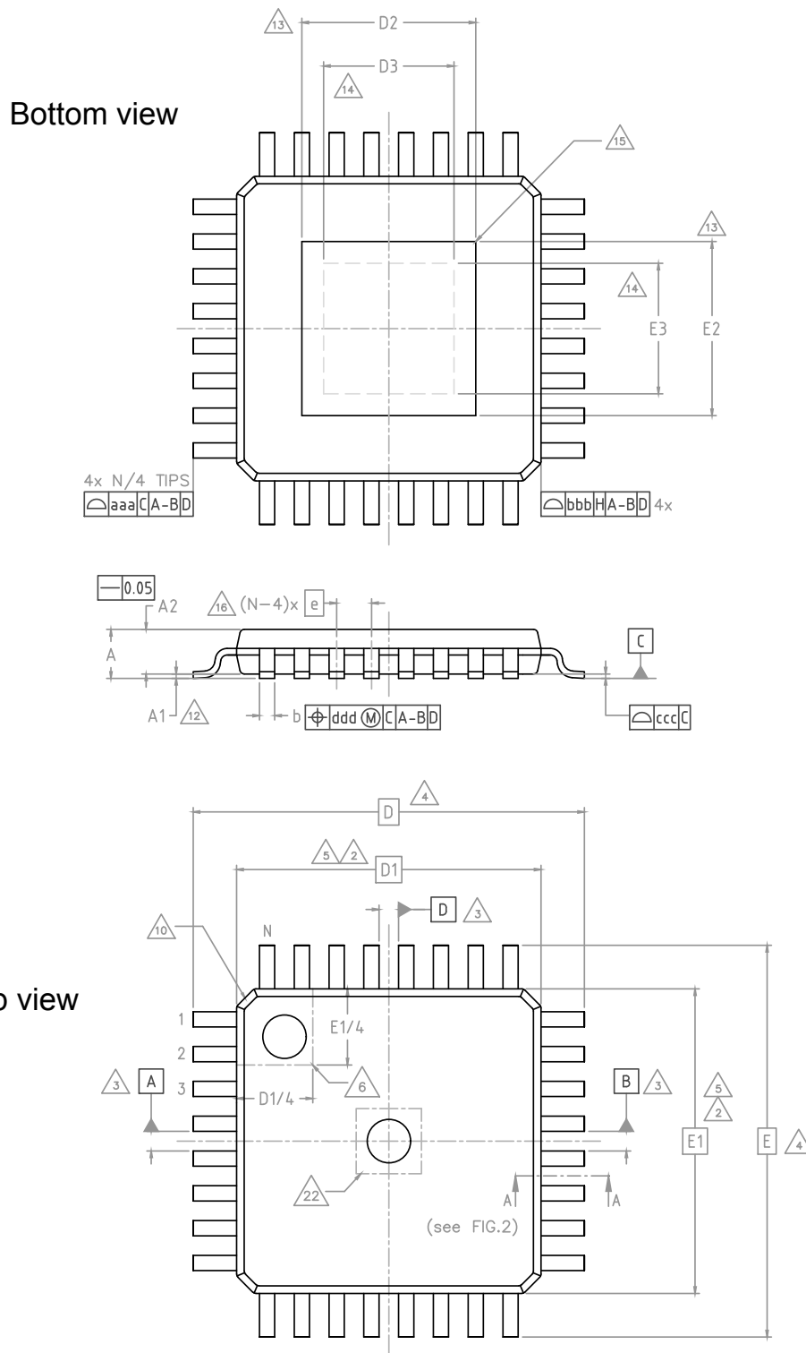
Figure 27. TQFP32L 7x7 mm package outline
