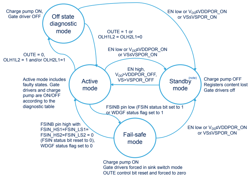
Figure 25. Operating modes
