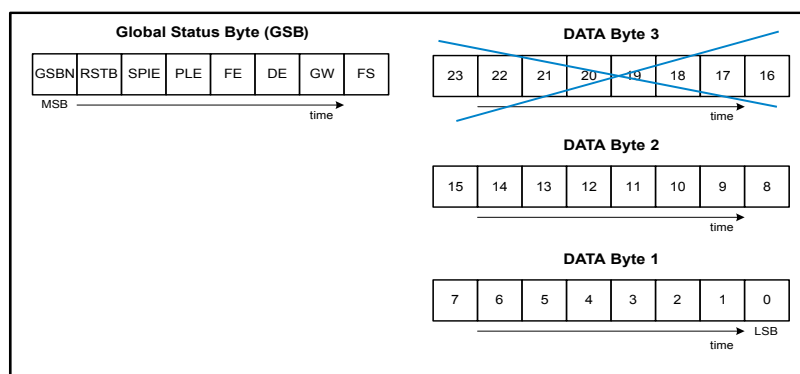
Figure 16. SDO frame
