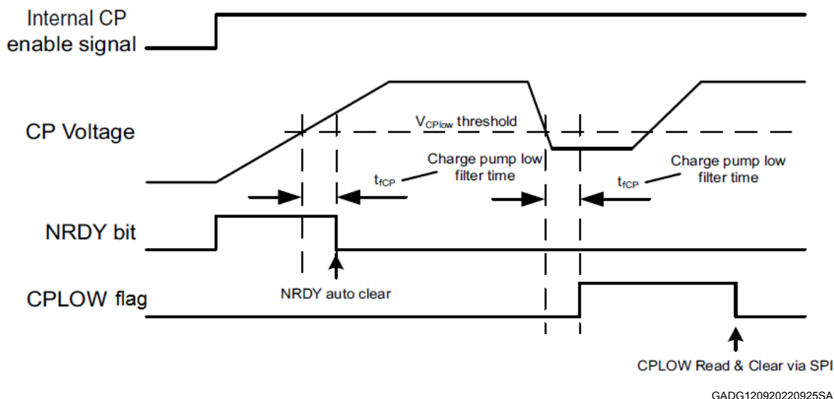
Figure 4. NRDY status bit and CPLOW flag
