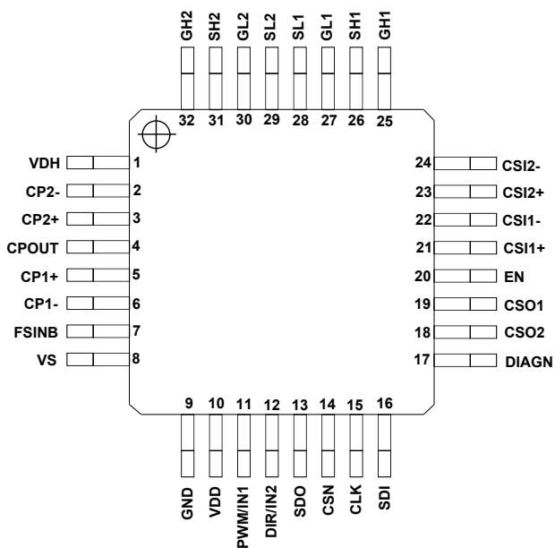
Figure 2. Pinout - TQFP32
