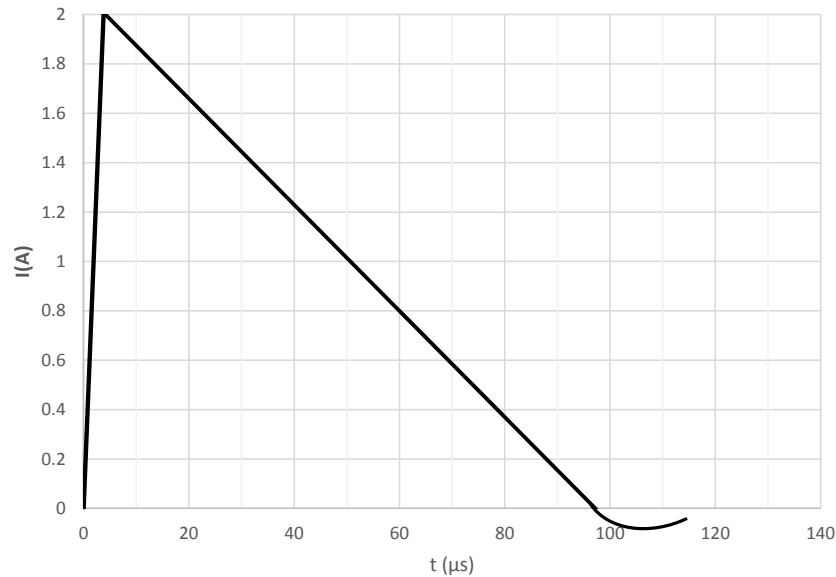
Figure 19. Surge waveform
