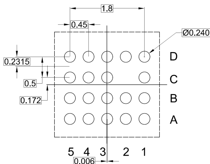
Figure 29. CSP19 Suggested footprint
