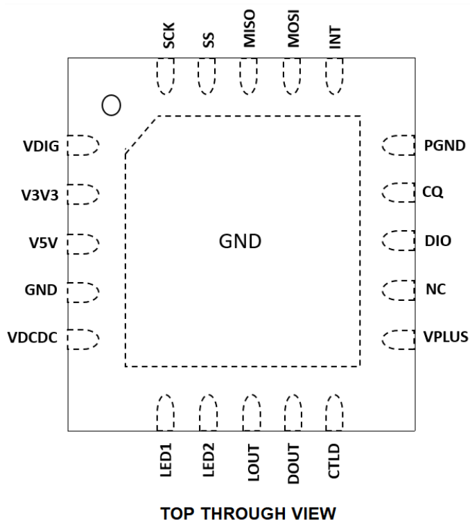
Figure 2. Package and pin-out - QFN
