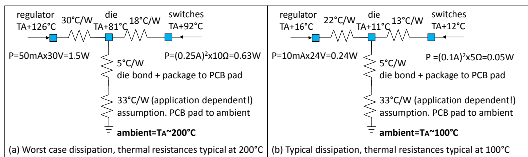
Figure 18. Example of thermal power dissipation estimation
