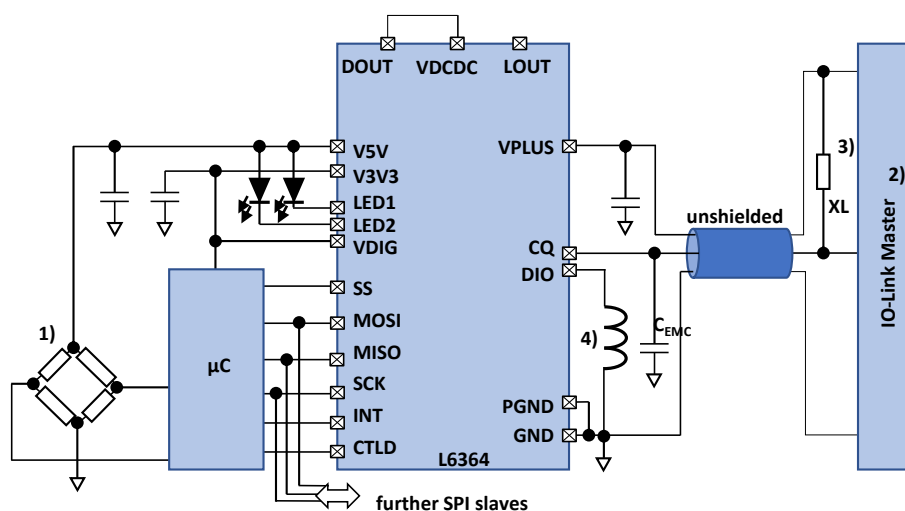
Figure 23. Application example: DC-DC disabled, CQ as line driver, DIO as load driver, V_{\text{SENSOR}} = 5.0 \text{ V} , V_{\text{MCU}} = \text{VDIG} = 3.3 \text{ V}
