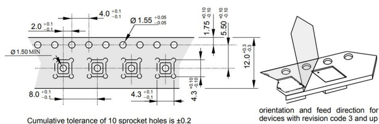
Figure 30. CSP19, Packing Information
