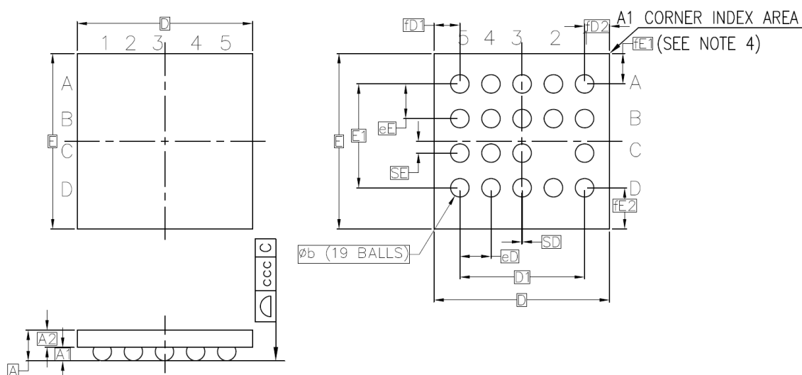
BOTTOM VIEW
