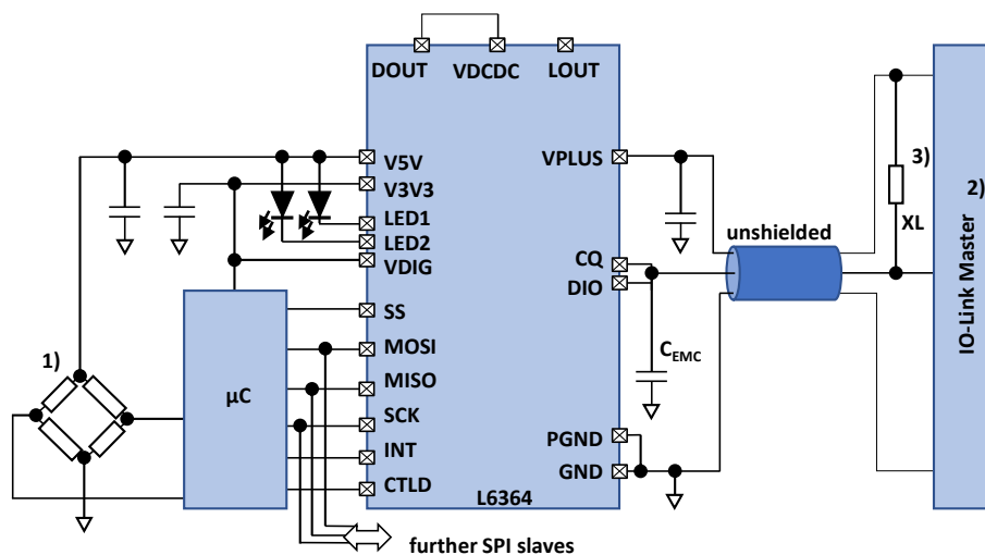
Figure 21. Application example: DC-DC disabled, CQ and DIO coupled (Join Mode), V_{\text{SENSOR}} = 5\text{ V} , V_{\text{MCU}} = V_{\text{DIG}} = 3.3\text{ V}
