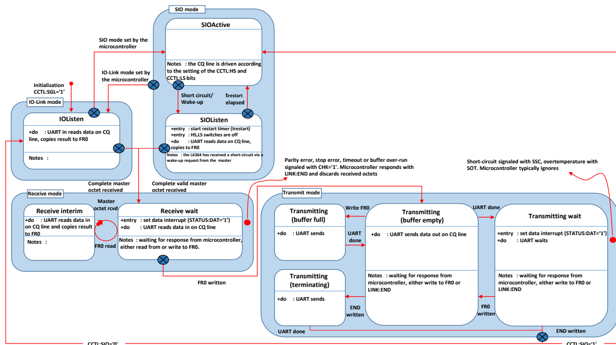
Figure 8. Single octet UART mode state diagram
