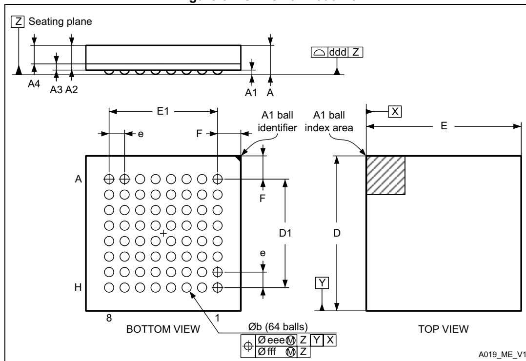
Figure 61. UFBGA64 - outline
