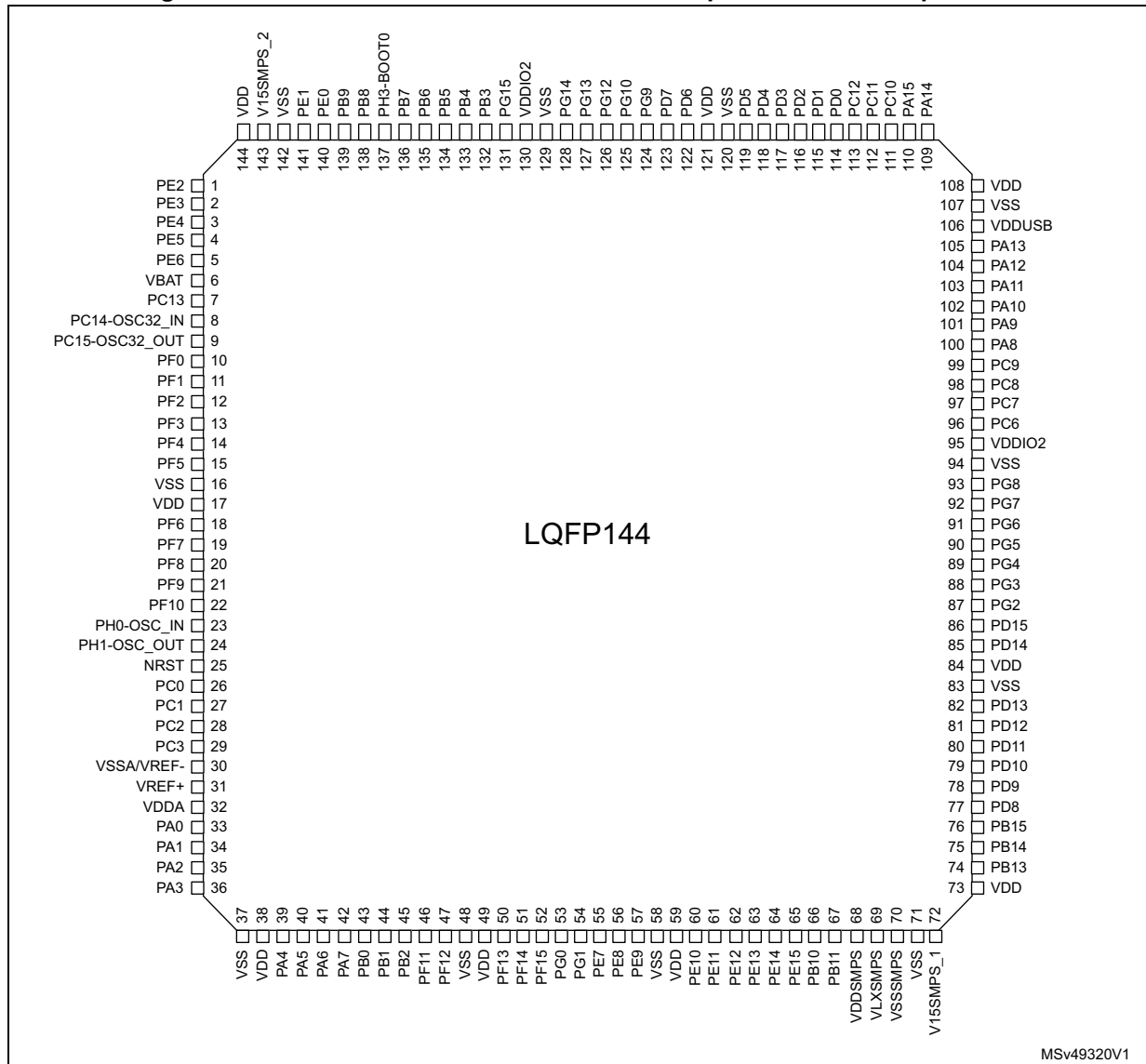
Figure 25. STM32L552xxxQ LQFP144 SMPS step down converter pinout (1)
