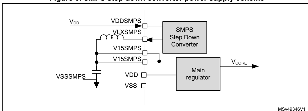
Figure 6. SMPS step down converter power supply scheme
