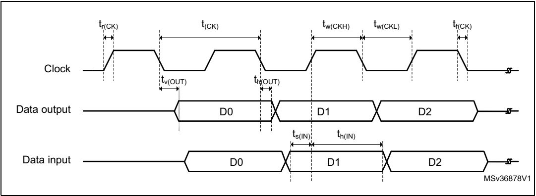
Figure 66. OCTOSPI timing diagram - SDR mode
