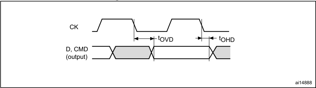
Figure 73. SD default mode
