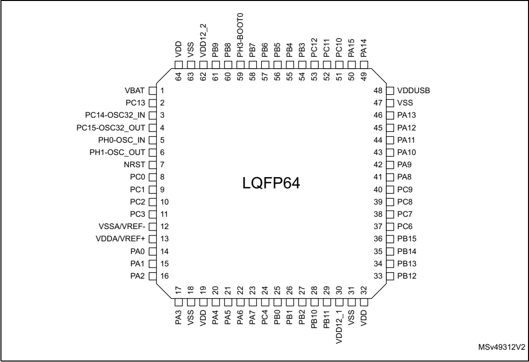
Figure 16. STM32L552xxxxP LQFP64 external SMPS pinout (1)
