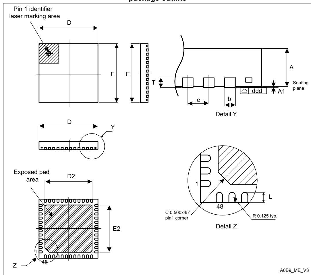
Figure 75. UFQFPN48 - 48-lead, 7x7 mm, 0.5 mm pitch, ultra thin fine pitch quad flat package outline
