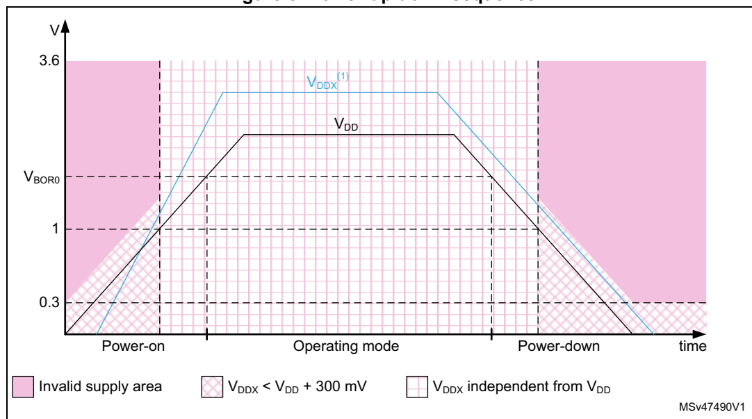
Figure 5. Power-up/down sequence
