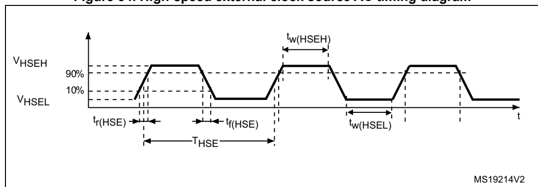
Figure 34. High-speed external clock source AC timing diagram
