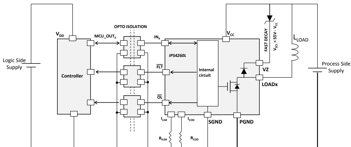
Figure 5. Application circuit (fast decay enabled by TVS between Vz and supply rail)
