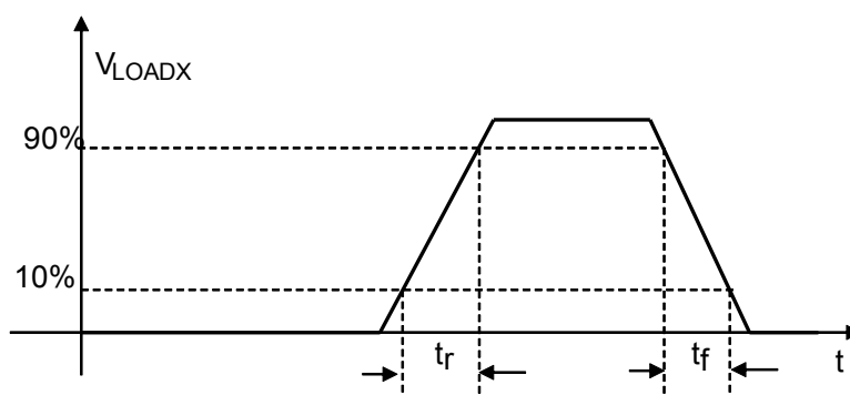
Figure 3. t_{rise} and t_{fall}
