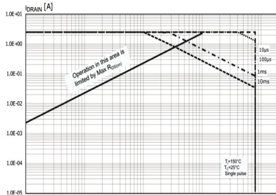
Figure 23. SOA SSOP10 package
