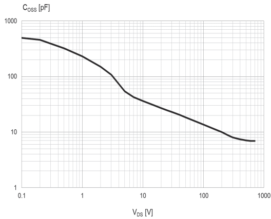
Figure 20. Power MOSFET capacitance variation vs VDS @ VGS=0, f=1MHz
