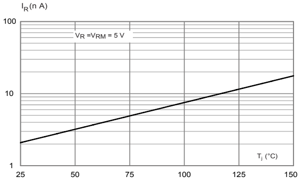
Figure 2. Variation of leakage current versus junction temperature
