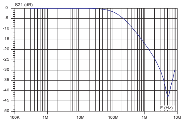
Figure 7. S21 attenuation
