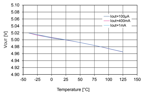
Figure 9. Output voltage vs. temperature ( V_{IN} = 4.3\ \text{V} , V_{OUT} = 3.3\ \text{V} )
