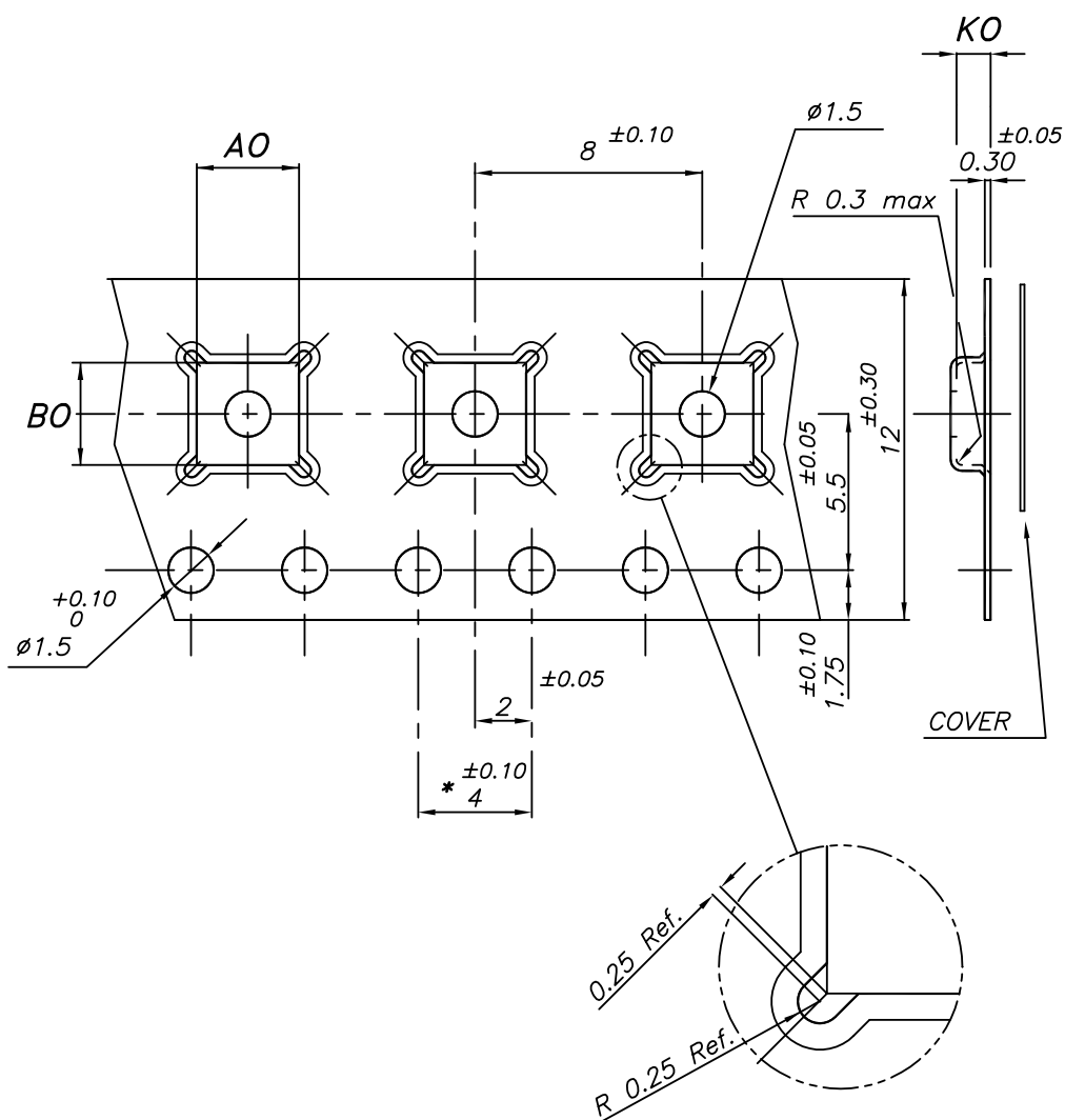
Figure 42. DFN6 (3x3) tape outline
