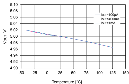
Figure 7. Output voltage vs. temperature ( V_{IN} = 13.2\ \text{V} , V_{OUT} adjusted to 5\ \text{V} )
