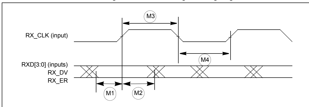
Figure 39. MII receive signal timing diagram
