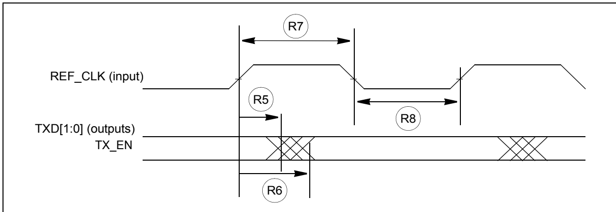
Figure 45. RMII transmit signal timing diagram
