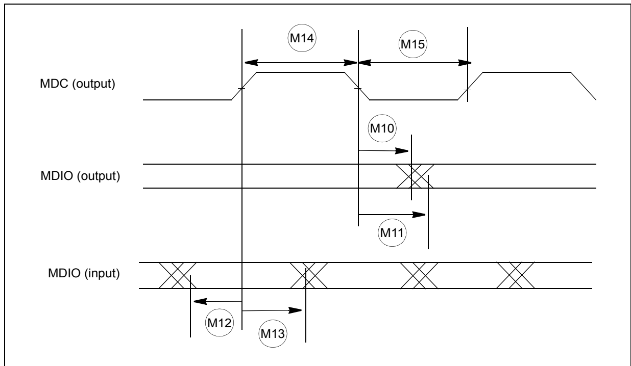
Figure 43. MII serial management channel timing diagram
