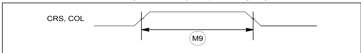
Figure 41. MII async inputs timing diagram
