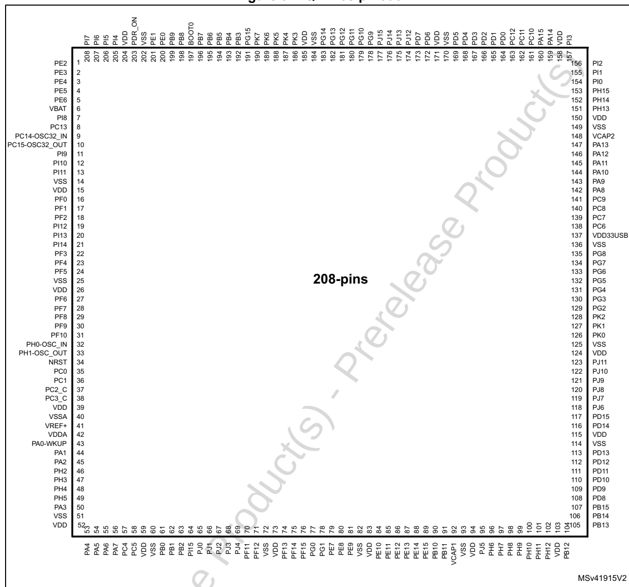
Figure 9. LQFP208 pinout
