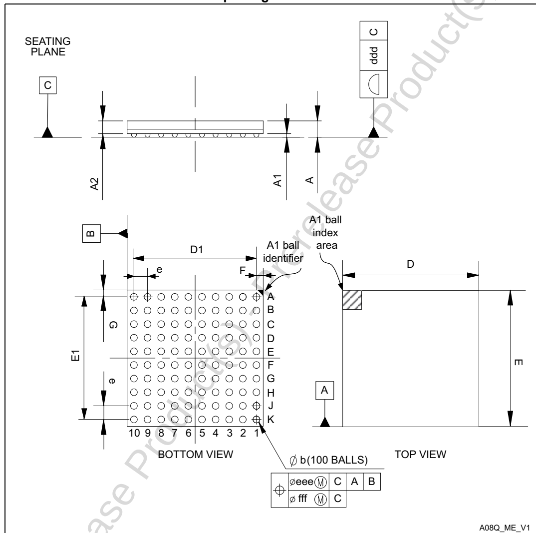
Figure 67. TFBGA100, 8 × 8 × 0.8 mm thin fine-pitch ball grid array package outline
