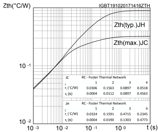
Figure 13. IGBT thermal impedance
