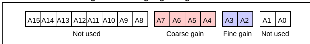
Figure 23. Analogue gain register format
