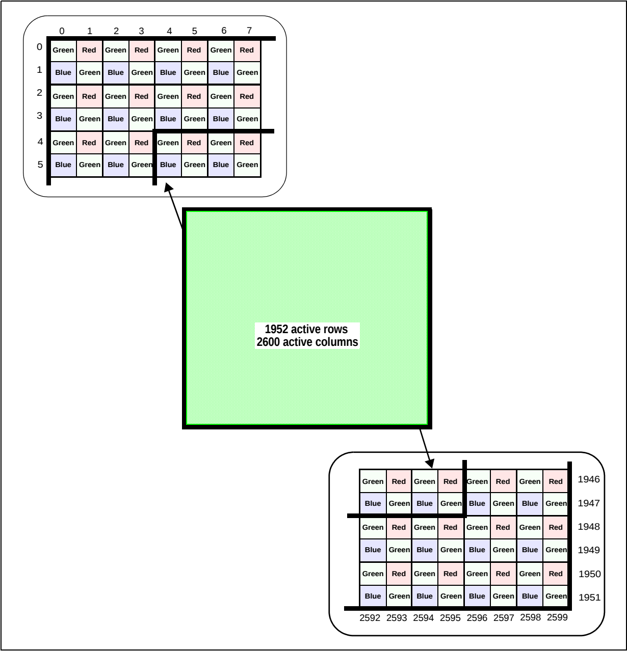
Figure 22. Bayer pattern
